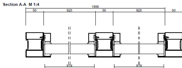
Typical standard profile
