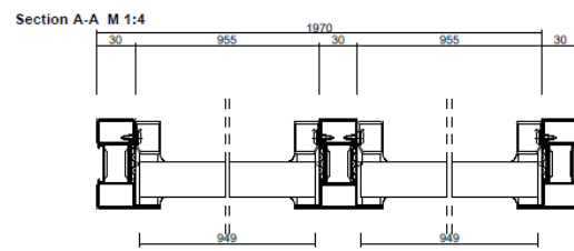
Typical slimline profile
